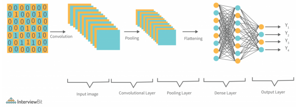
Figure 3 (CNN Layered Structure)
